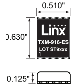
Figure 1: Package Dimensions
