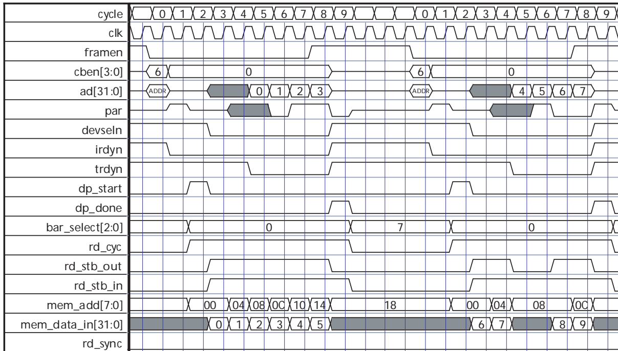
Figure 24 • FIFO Recovery Operation (RD_SYNC = 0)
