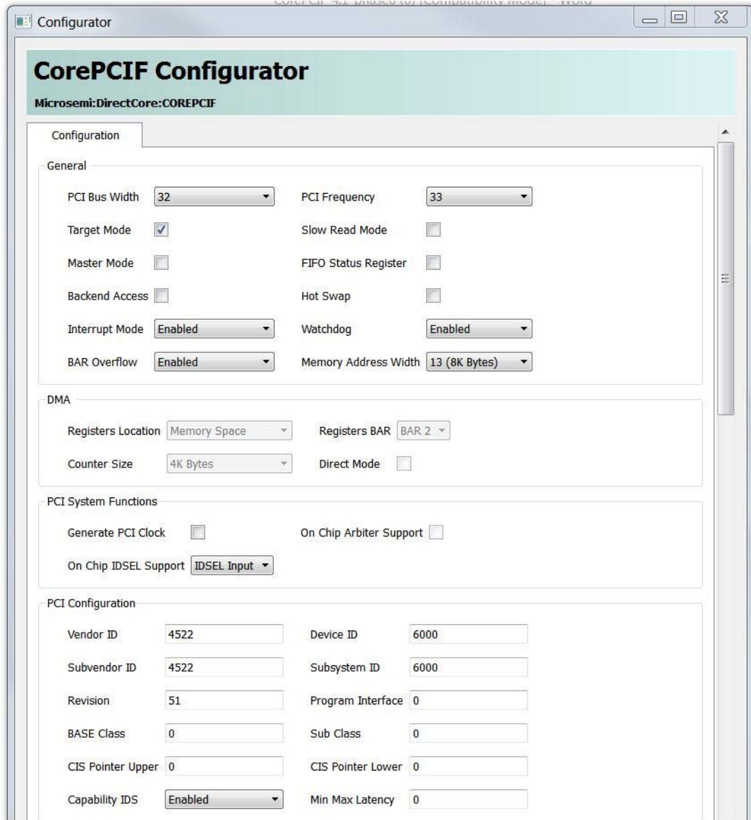
Figure 9 • CorePCIF Configurator
