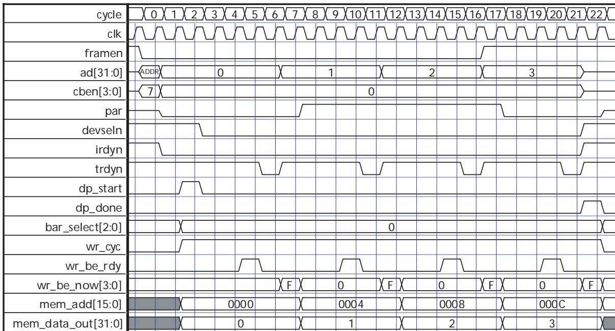
Figure 22 • Backend Burst Write Cycle with Slow Backend
