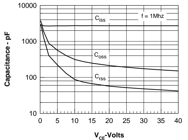
Fig. 6. Capacitance Curves
