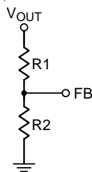
Figure 4. Setting V_{OUT} with a Resistive Voltage Divider
