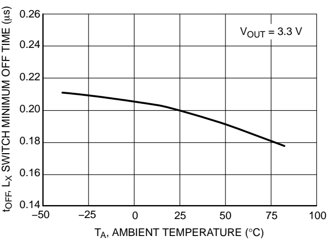
Figure 14. L X Switch Minimum OFF Time vs. Temperature
